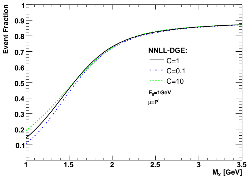
Figure 9: The event fraction R_{\text{cut}} within the range P^+P^- < M_X^2 and E_l > 1 GeV, computed using eq. (D.11) and eq. (3.53), plotted as a function of the cut value M_X . Different assignments for the unknown parameter C , which controls the shape of the perturbative quark distribution function (see eq. (3.29)) are used. In the matching coefficient the renormalization scale \mu = P^- is chosen.
