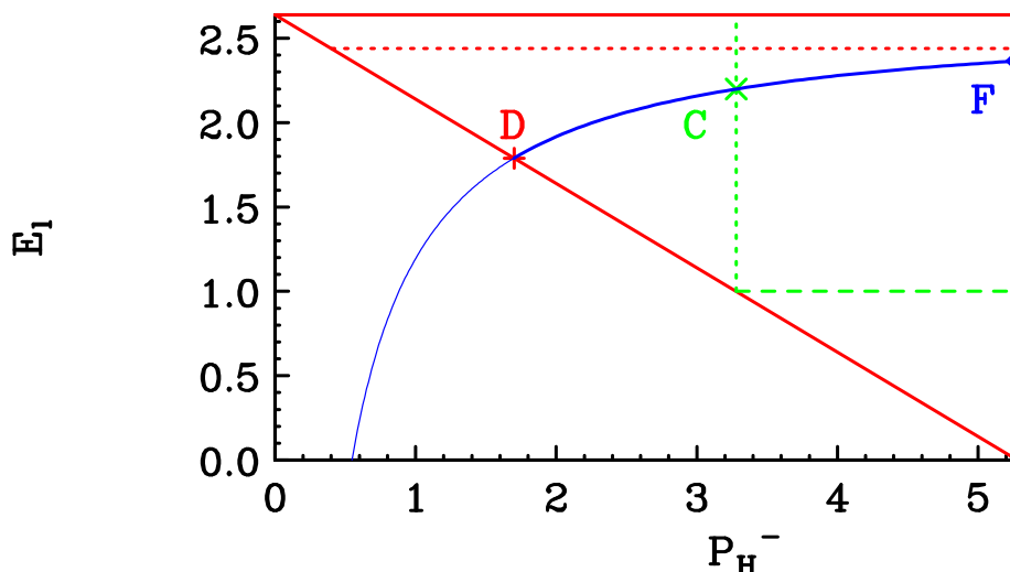
Figure 4: The full phase space in the (P^-, E_l) plain (upper left triangle) after the P^+ integration has been performed. The dotted horizontal line E_l = m_b/2 starting at P_H^- = \bar{\Lambda} is the upper boundary of the partonic phase space. A lower cut on the charged lepton energy (here E_l > E_0 = 1 \text{ GeV} ) removes the small triangular region below the horizontal dashed line. An upper cut on the hadronic invariant mass (here P^+P^- < M_X^2 = (1.7 \text{ GeV})^2 ) affects the distribution for E_l < \frac{1}{2}(M_B - M_X^2/P^-) . A full line separates between this region and the rest of the phase space where this cut is irrelevant. On this line we denoted three special points by D ( P^- = M_X ), C ( P^- = M_B - 2E_0 ) and F ( P^- = M_B ), respectively.
